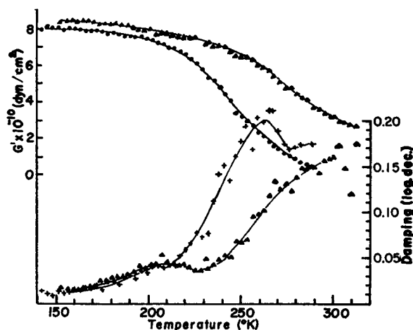
FIGURE 2 Dynamic shear behavior of shrunken collagen at 0.3-1 cps. \Delta , dry; + and \bullet , 10% H_2O .
